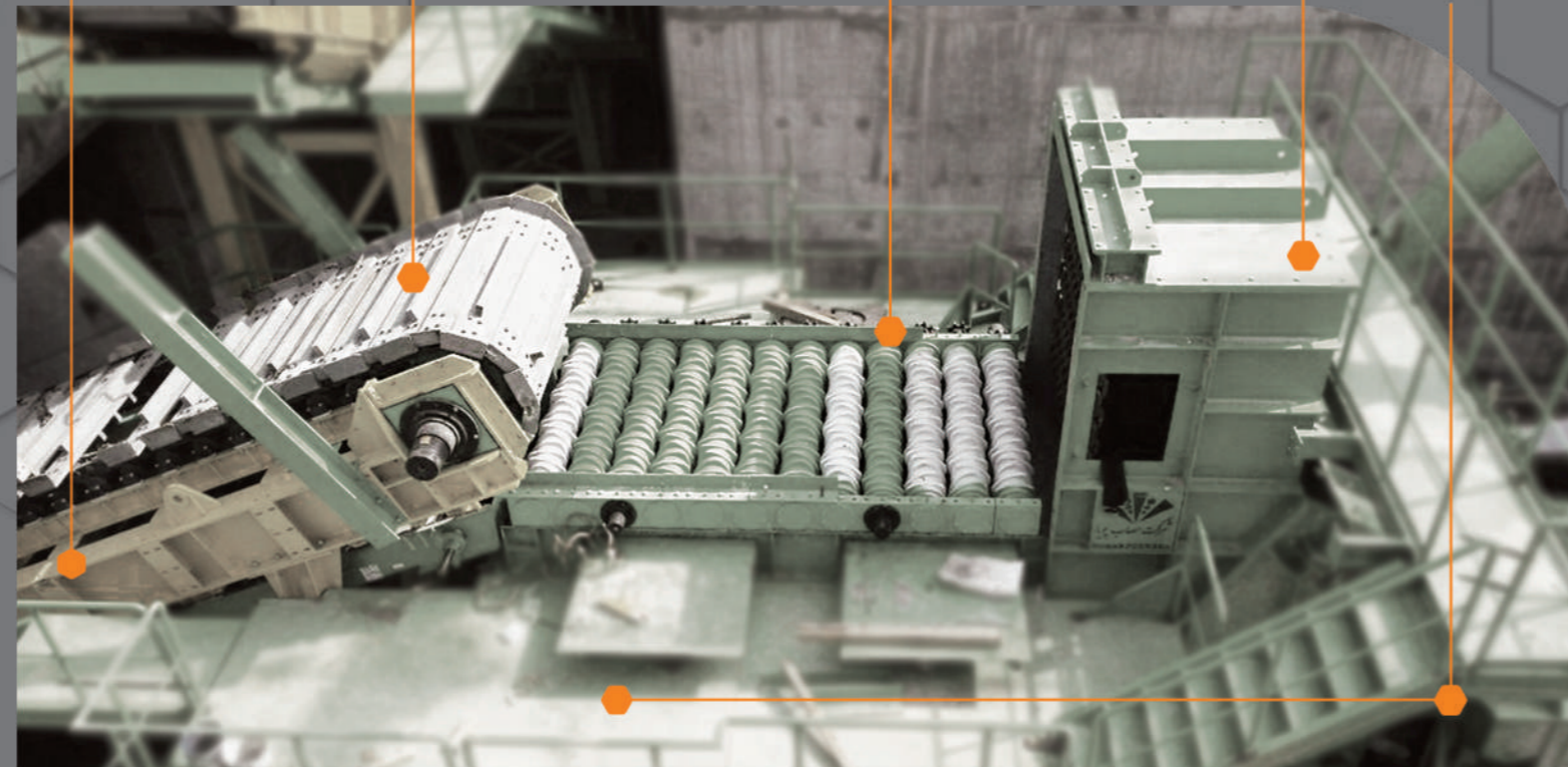
Apron Feeder's pan
