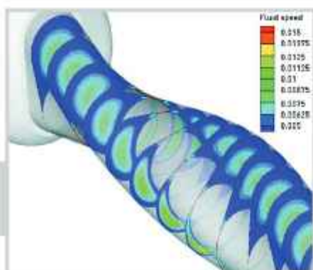
Pump dynamic numerical simulation
